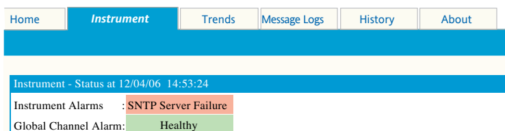
Figure C3.1 Affichage appareil
