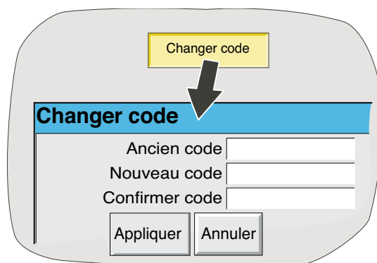
Figure 4.4.5 Changer code
