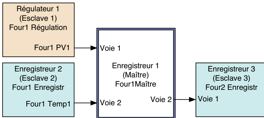
Figure 4.3.16j Configuration requise
